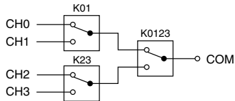
Figure 4. NI 2594 Power-On State
