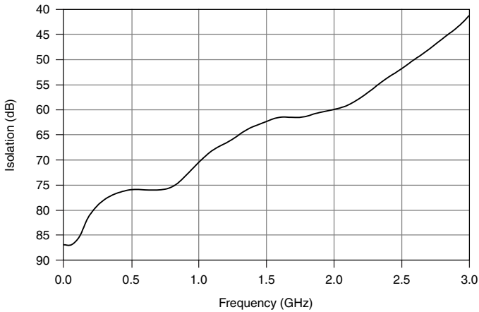
Figure 3. Typical Isolation
