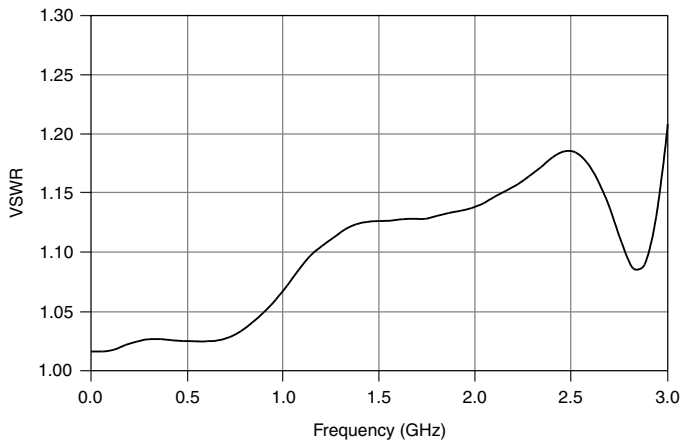
Figure 2. Typical VSWR
